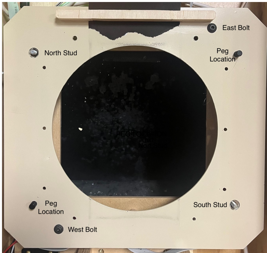
Figure 1: Component Location
